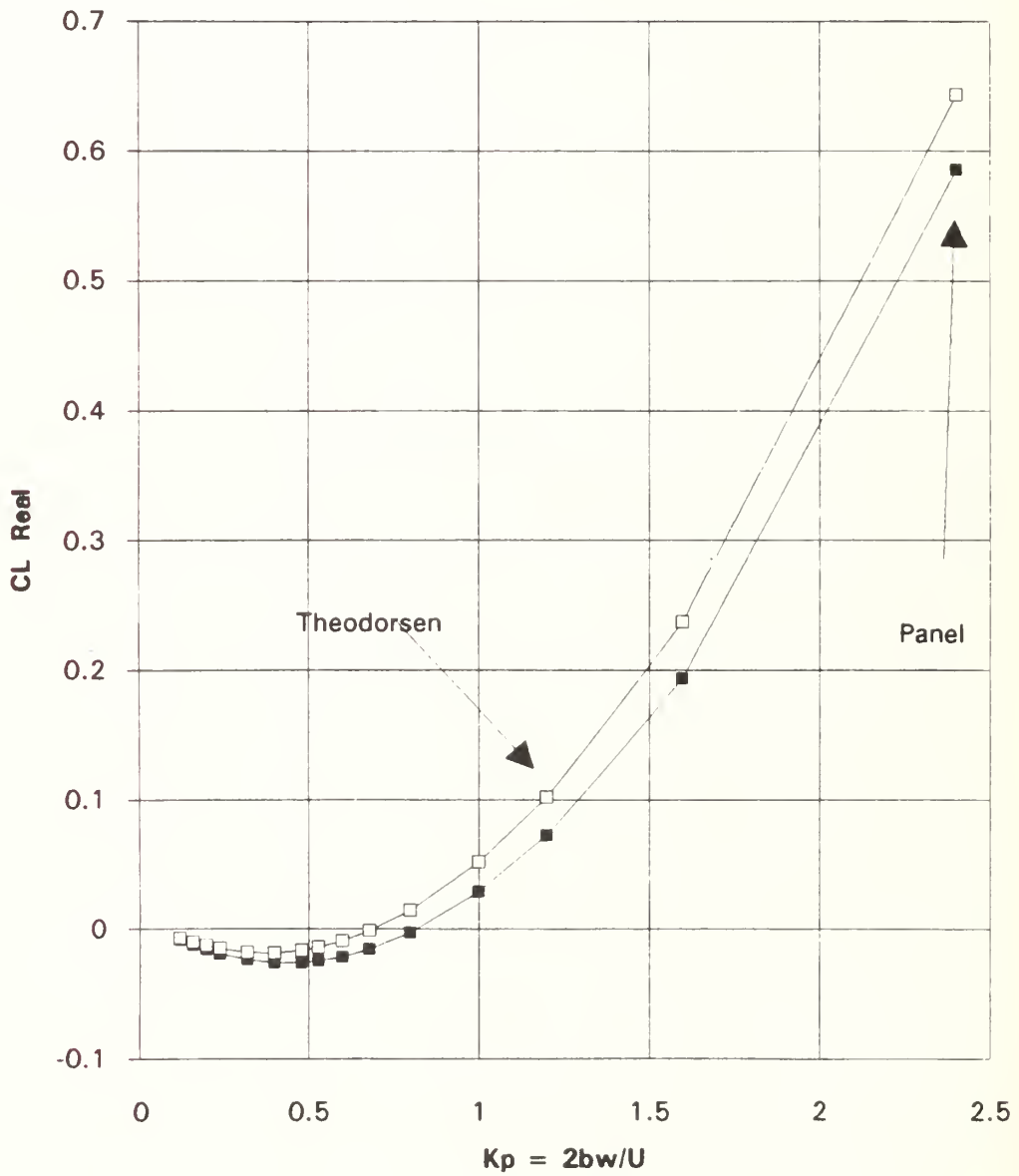
Real Part of CI for Panel and Theodorsen (plunge, .0833 h/2b, .37c, NACA0007,75 panels top and bottom, 3cycles of 65 calculations)
